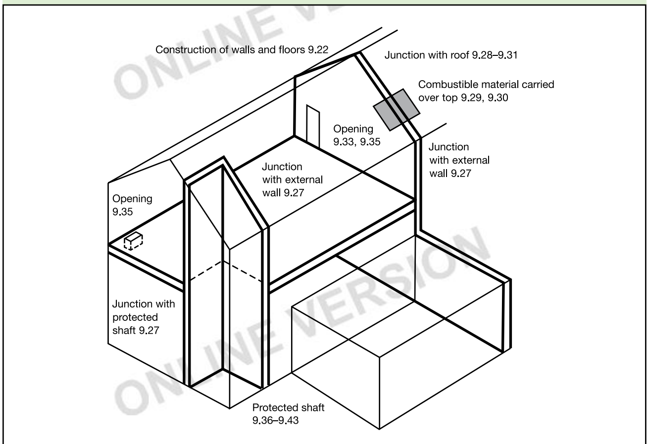
Diagram 27 Compartment walls and compartment floors with reference to relevant paragraphs in Section 9
