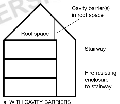
Diagram 33 Alternative arrangements in roof space over protected stairway in a house with a floor more than 4.5m above ground level
