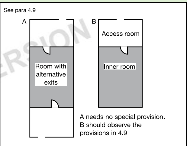
Diagram 17 Inner room and access room
