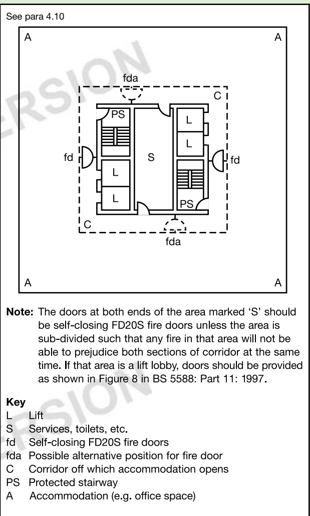
Diagram 18 Exits in a central core
